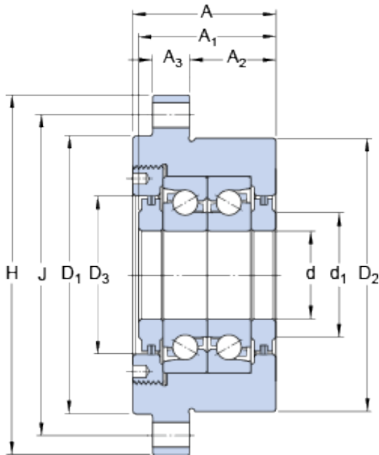
FBSA 209/DB Bearing 2D drawings and 3D CAD models
